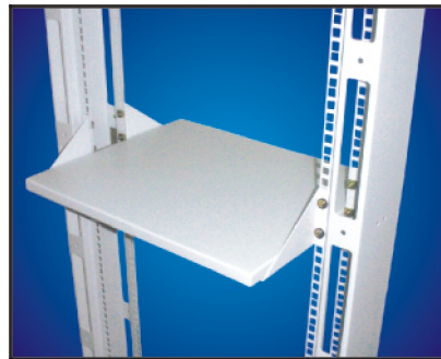
CFT37 - Open Rack Fixed Shelf 370mm Deep, 50kg Loading
