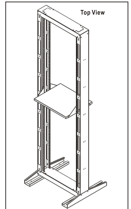
CF Class 42U 600 mm Wide Open Rack
